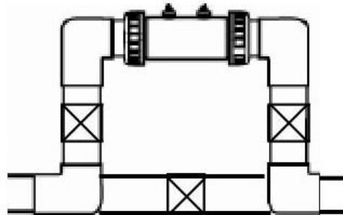
Installation with bypass
